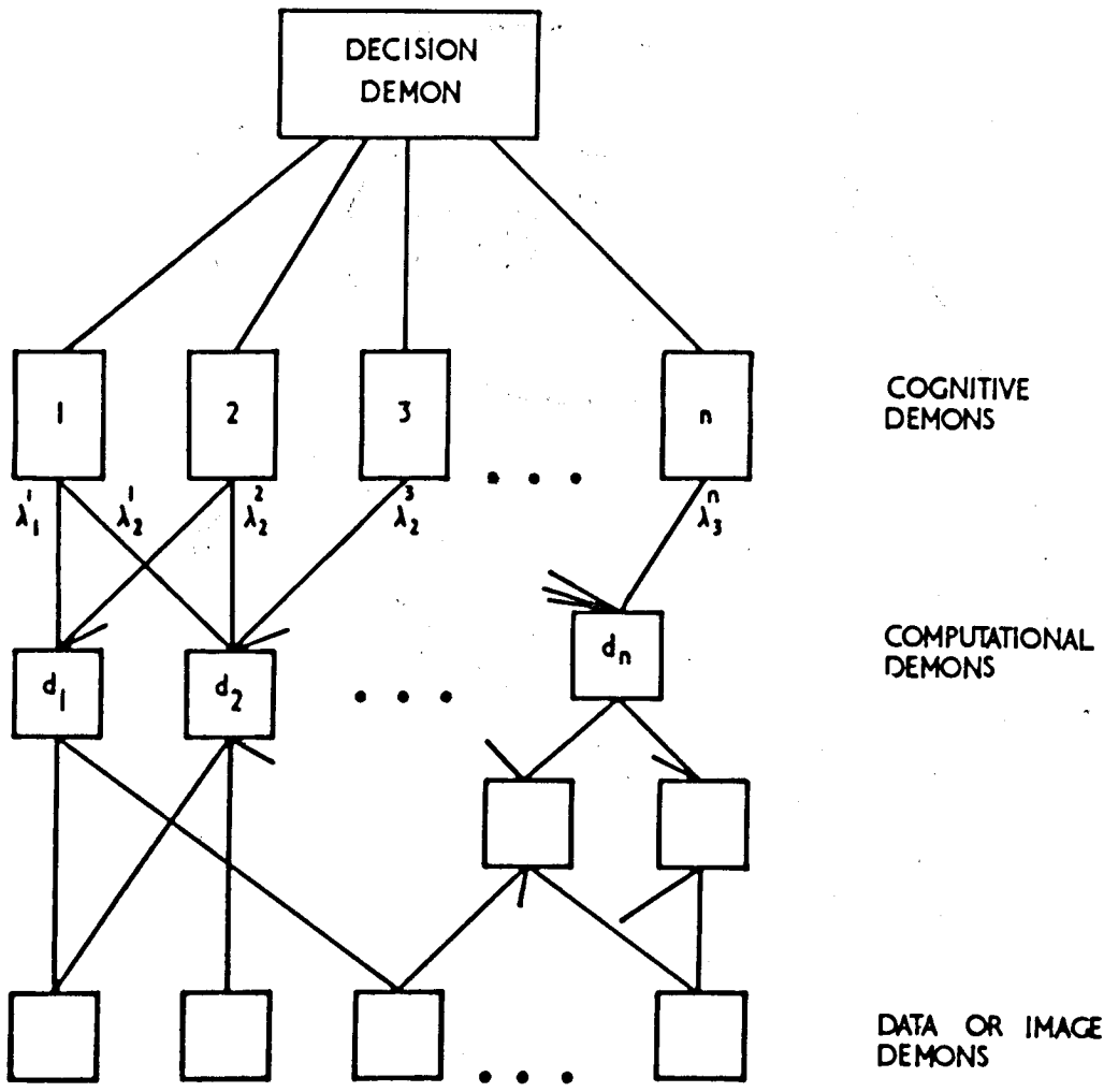
Fig. 3. Amended Pandemonium
