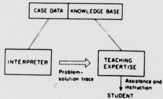
FIG. 2. Modules for a multiple-domain tutorial system.
