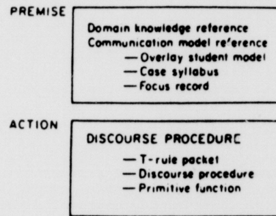
FIG. 3. Form of a tutorial rule
