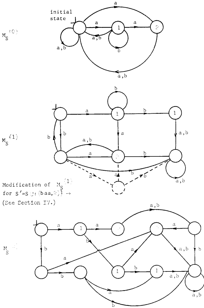
Fig. 1. M_S^i for i=0, 1, 2 and S = \{(a, 1), (aa, 2), (ab, 1), (ba, 2), (aba, 2), (abb, 1), (bba, 1), (aaaa, 2), (aaba, 2)\} .
