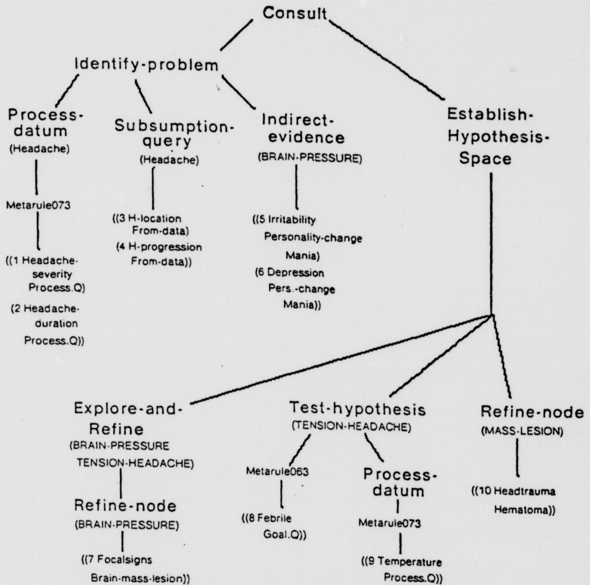
Figure 4-1: 10 explanations of student planning, resolved into a global plan (Boldface nodes are tasks invoked by NEOMYCIN meta-rules; small capitals denote active hypotheses; numbers are followed by student's data query; remaining terms refer to kinds of strategies and contexts)
