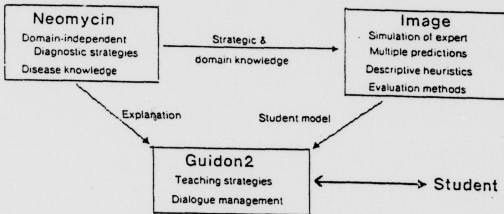
Figure 1-1: Components of the GUIDON2 teaching system
