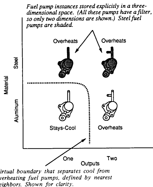
Figure 6. Schematic of the representation used in nearest neighbor learning methods. Instances are stored explicitly in a space of N dimensions, where each dimension describes one feature of the instance. The figure depicts the two-dimensional case. To classify an instance, one finds the nearest stored instance and predicts its class. It is possible to define a decision boundary representing equal distance from stored instances of different classes (shown as a curved line in the middle of the figure). Typically these decision boundaries are not stored explicitly.
