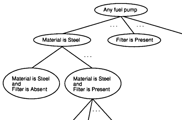
Search moves from general rule conditions to specific ones until the matching pumps are not statistically distinguishable.
