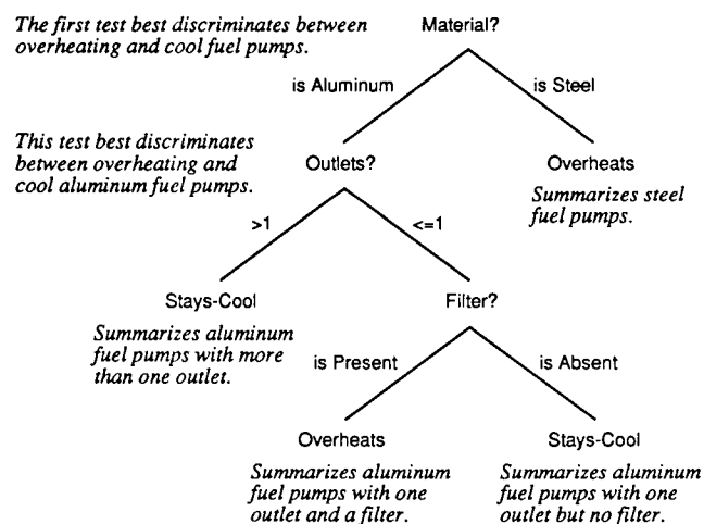
Figure 4. Schematic of the representation and search used in decision tree learning. To classify an instance, the test at the root of the tree (shown at top) is applied first, and based on the outcome, classification proceeds with the appropriate subtree. The search begins by determining the single most discriminating test. Instances are then partitioned by their outcome for this test. The standard method terminates search when all instances in a partition are of the same class (or there are no more tests), but some variants use statistical tests to halt earlier as an effort to avoid overfitting.
