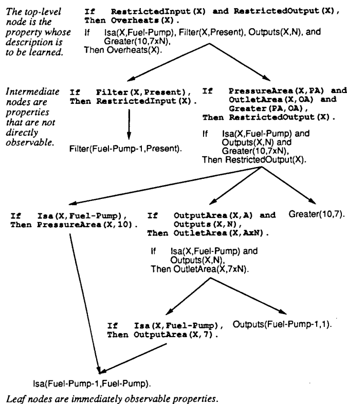
Figure 5. Schematic of the representation used by explanation-based generalization. Properties of an instance (depicted as leaves) and domain knowledge encoded as rules (depicted in teletype font) justify or explain other properties of the instance that may not be immediately observable. By extracting the weakest preconditions under which this justification holds, one can construct rules that are more general than the specific instance but more special than the general domain knowledge rules (depicted below each domain knowledge rule in sans-serif font). These rules allow inferring a non-observable property by testing only immediately observable properties of an instance.
