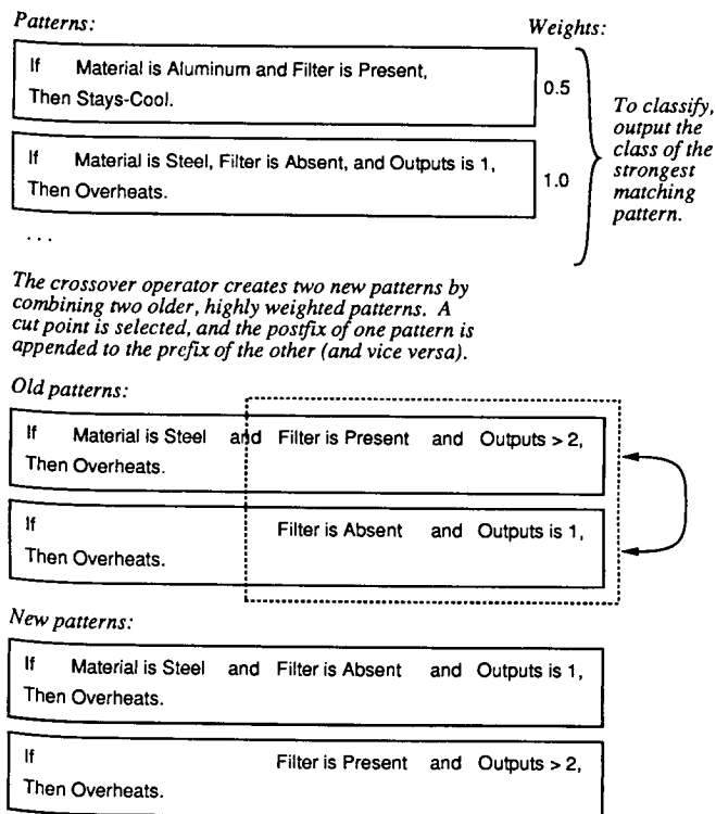
Figure 2. Schematic of the representations and operators used in the genetic algorithm. The weights of conjunctive patterns (shown at top) are used to classify instances. Learning modifies both the weights of patterns and their conditions. The simplest operator generates new patterns that are minor random variations of old ones (not shown). The crossover operator (shown at bottom) splices together an arbitrary prefix of one pattern with an arbitrary suffix of another (and vice versa).
