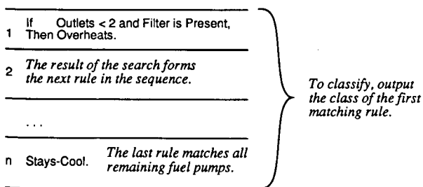
Figure 3. Schematic of the representation and search used in CN2, a recent rule learning method. Learned rules (shown at bottom) are ordered, with the last rule identifying the class of any remaining instances. Search maintains a limited size boundary as it looks for rule conditions that are both predictive and reliable. Initially, it looks for a consistent description of a single class given all the instances, and subsequently it searches for a consistent description of those examples not covered by any rules found thus far. Search terminates when all instances are covered by some rule.
