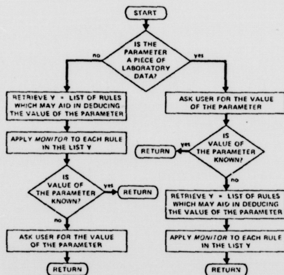
Fig. 2. Flow chart describing the FINDOUT strategy for determining which questions to ask the user. The derivation of values of parameters may require recursive calls to the MONITOR , thus dynamically creating a reasoning chain.
