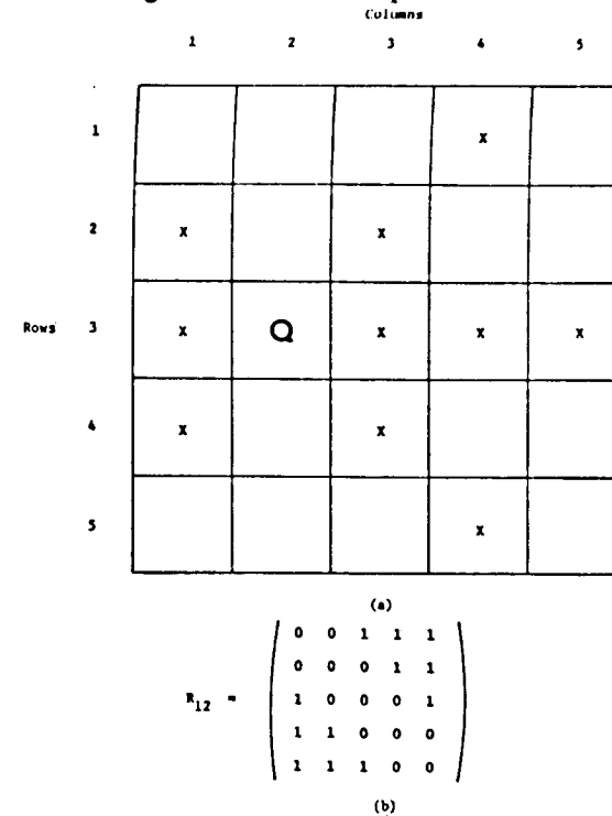
FIG. 3. Illustrating the 5-queens problem.
