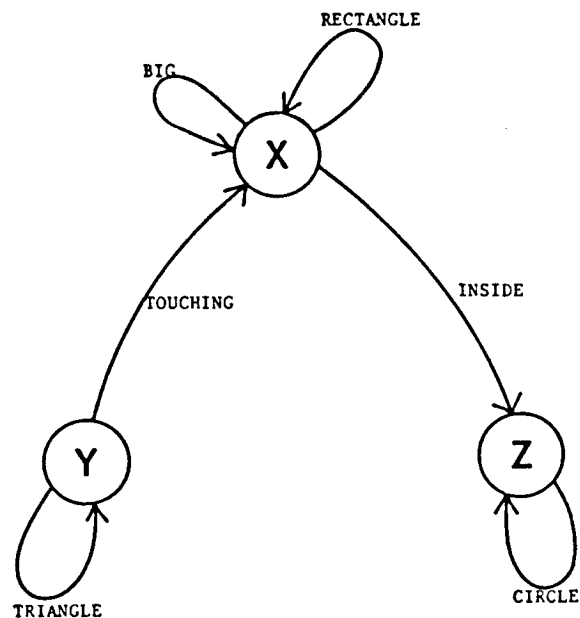
FIG. 5. A network representation of a retrieval task.
