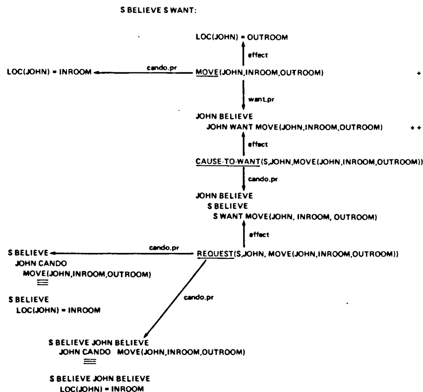
Figure 2. A plan for a REQUEST.
