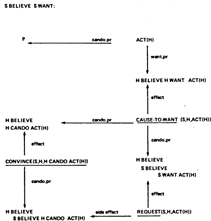
Figure 8. A REQUEST with side effects.
