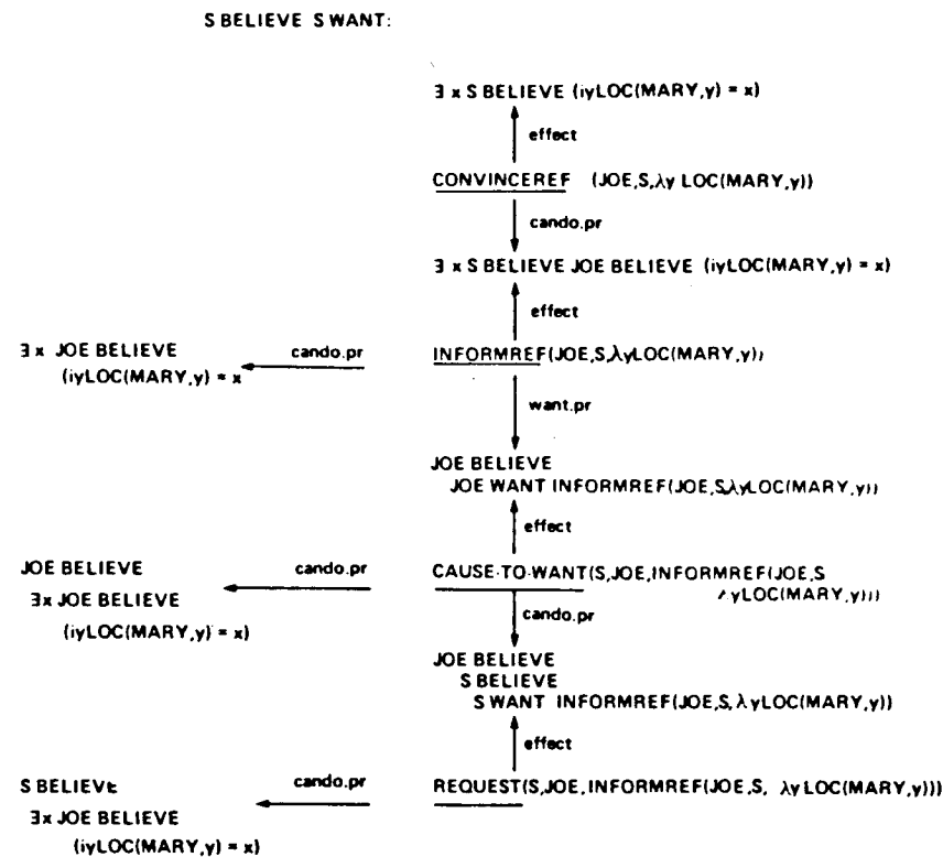
Figure 5. A plan for a wh-question.
