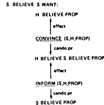
Figure 3. A plan for an INFORM.
